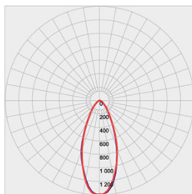
Candle Power Distribution
