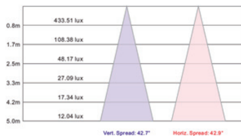
Illuminance at a Distance
