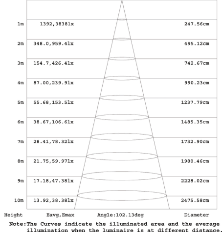
Flux out:6911 lm
